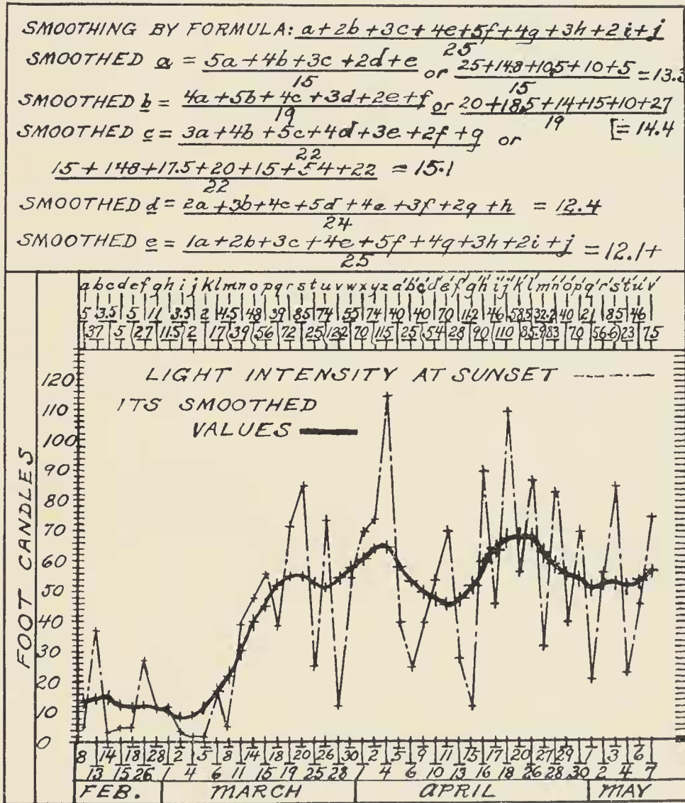
FIG. 5. The Method of Smoothing Curves.
